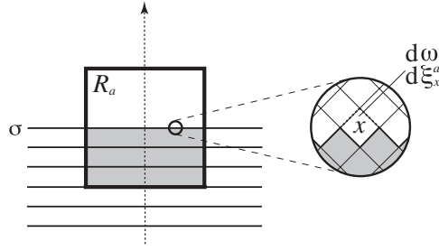
Figure 2. The diagram represents a sequence of spacelike hypersurfaces advancing through the spacetime region R_a . The grey shading within R_a corresponds to the spacetime volume \omega_\sigma^a . The detail shows a small spacetime region within R_a where the surface \sigma advances through a spacetime cell at point x . Associated with the cell at point x is the incremental spacetime volume d\omega and the incremental Brownian variable d\xi_x^a .
